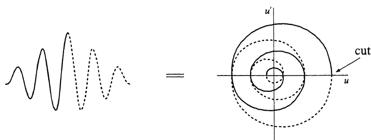
Figure 2. The statement of theorem 1: when the curve is cut at \bar{x} , the two resulting curves do not self-intersect.
